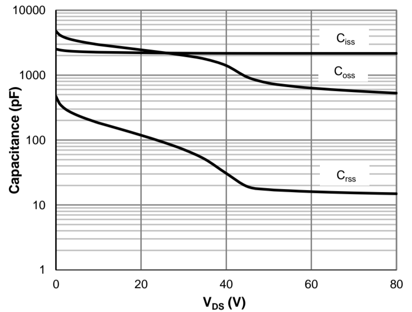
Figure 8: Capacitance Characteristics
